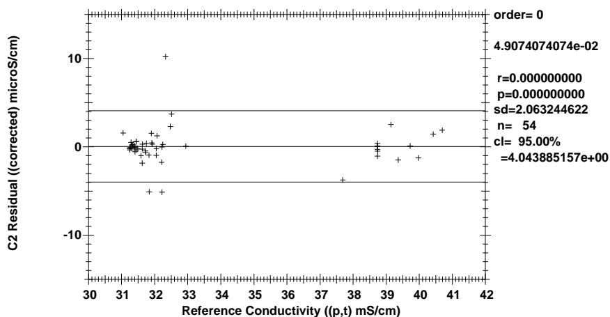
Figure 1.4.3.5 MV1310 Corrected C Bottle - C2 by conductivity (-0.01°C ≤ T1-T2 ≤ 0.01°C).
