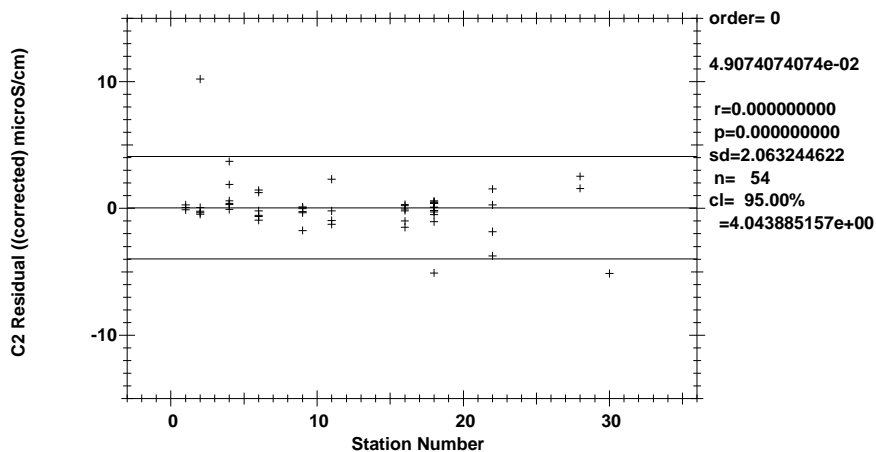
Figure 1.4.3.2 MV1310 Corrected C Bottle - C2 by station (-0.01°C ≤ T1 - T2 ≤ 0.01°C).
