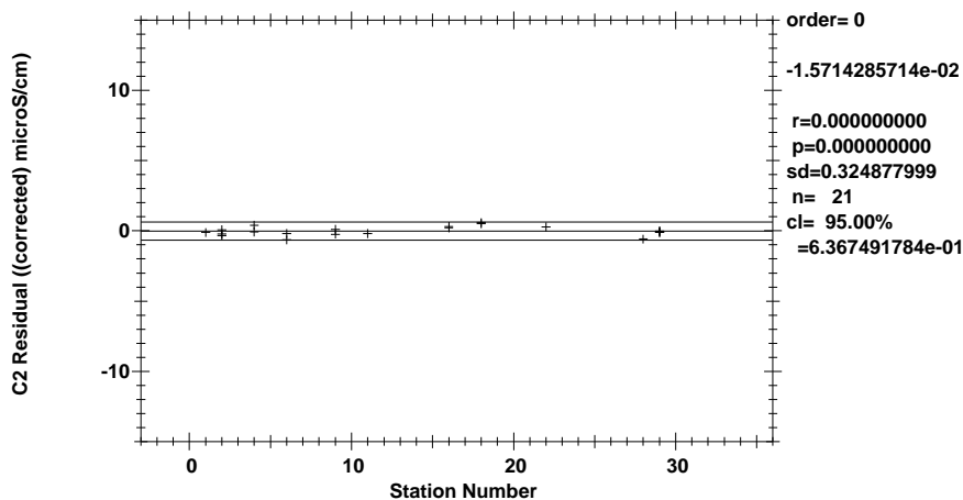
Figure 1.4.3.3 MV1310 Deep Corrected C Bottle - C2 by station (Pressure ≥ 1800 dbars).
