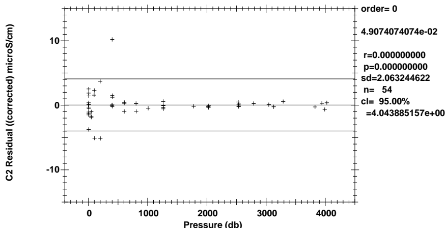
Figure 1.4.3.4 MV1310 Corrected C Bottle - C2 by pressure (-0.01°C ≤ T1-T2 ≤ 0.01°C).
