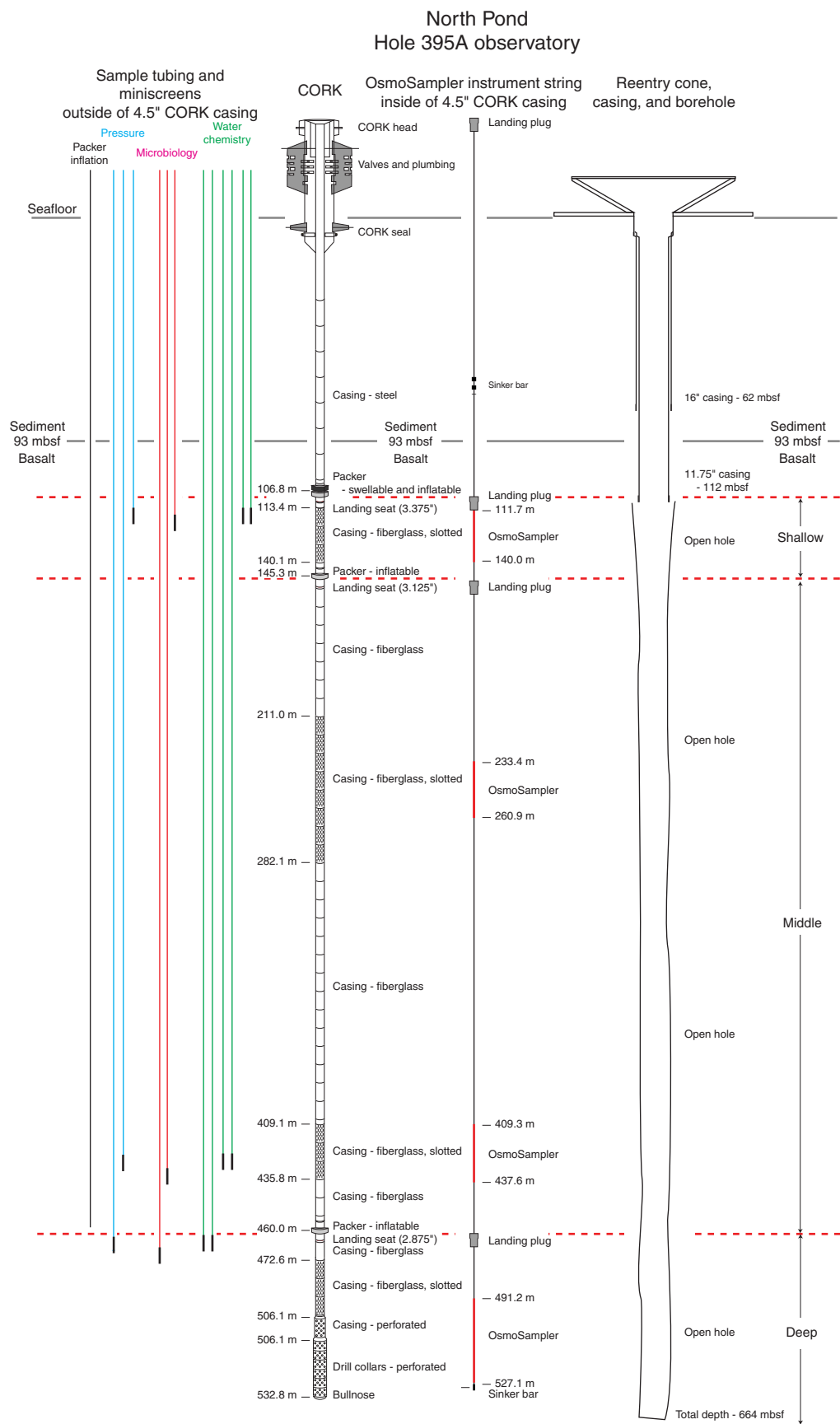
Figure F4. Configuration of the primary parts of the new subseafloor borehole observatory (CORK) deployed in Hole 395A.
